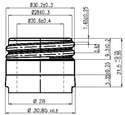
MINIMUM THROUGH BORE - Ø 18 FINISH DETAILS (SCALE 2:1)
